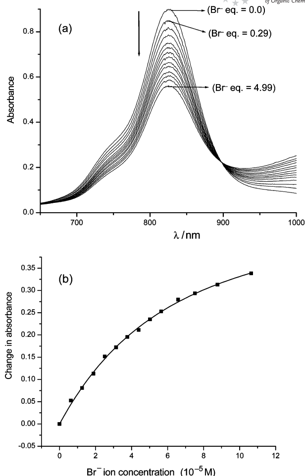
Figure 4. a) UV/Vis titration curve for protonated dithiaphlorin 6\cdot\text{H}^+ with increasing amounts of tetrabutylammonium bromide salt in dichloromethane. b) The curve-fitting plot of the change in absorbance ( \Delta A ) vs. the concentration of \text{Br}^- anion. The concentration of the dithiaphlorin used was 2.13 \times 10^{-5} M and the concentration range of the \text{Br}^- used was 6.29 \times 10^{-6} M to 1.06 \times 10^{-4} M. The spectra were measured at 825 nm at 22 °C.
