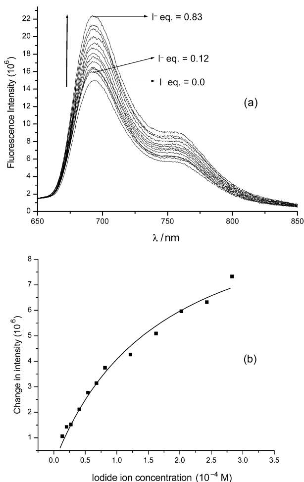
Figure 5. a) Fluorescence titration of thiaphlorin-porphyrin dyad 27\cdot\text{H}^+ with increasing amounts of tetrabutylammonium iodide in dichloromethane. b) The curve fitting plot of the change in fluorescence intensity ( \Delta I ) vs. the concentration of \text{I}^- anion. The 8.82 \times 10^{-6} M dichloromethane solution of dyad 27 was selectively protonated by addition of 1.5 \mu\text{L} of 2 \times 10^{-3} M trifluoroacetic acid in dichloromethane (the TFA concentration was 9.67 \times 10^{-7} M). The dyad 27\cdot\text{H}^+ was excited at 520 nm and the concentration range of iodide salt used was 1.06 \times 10^{-6} M to 7.32 \times 10^{-6} M.
