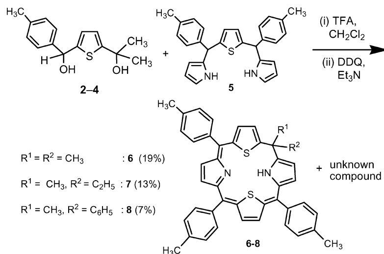
Scheme 5. Synthesis of 21,23-dithiaphlorins 6–8 .
