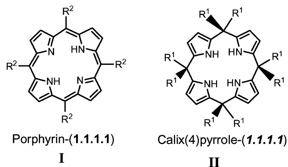
Scheme 1. Structures of porphyrins and calix(4)pyrroles.
