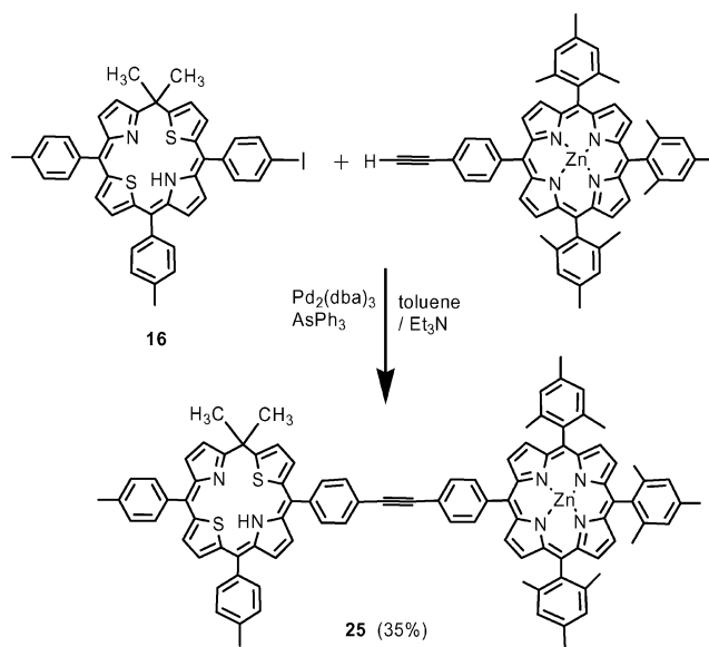
Scheme 10. Synthesis of covalently linked 21,23-dithiaphlorin–porphyrin dyad 25 .
