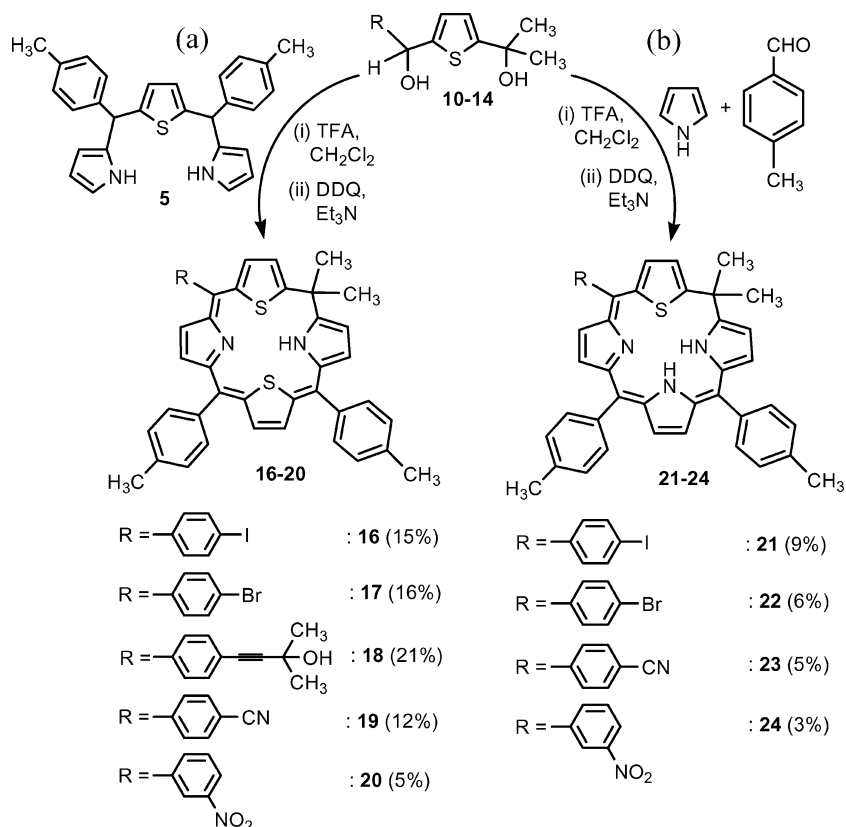
Scheme 8. Synthesis of monofunctionalized 21,23-dithiaphlorins 16–20 and 21-thiaphlorins 21–24 .
