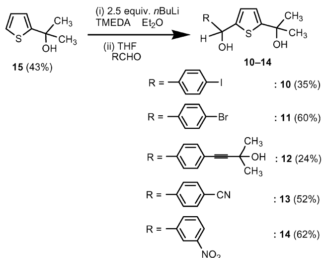
Scheme 7. Synthesis of functionalized unsymmetrically substituted 2,5-thiophenedimethanols 10–14 .
