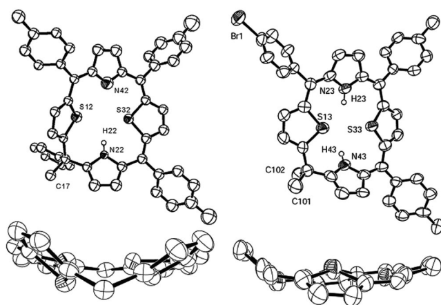
Figure 2. X-ray crystal structures of a) 8 and b) 17·H + . Thermal ellipsoids are shown at the 50% probability level. In the bottom view, meso aryl groups have been removed for clarity.
