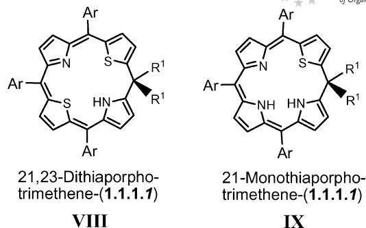
Scheme 3. Structures of 21,23-dithia- and 21-thiaphlorins.
