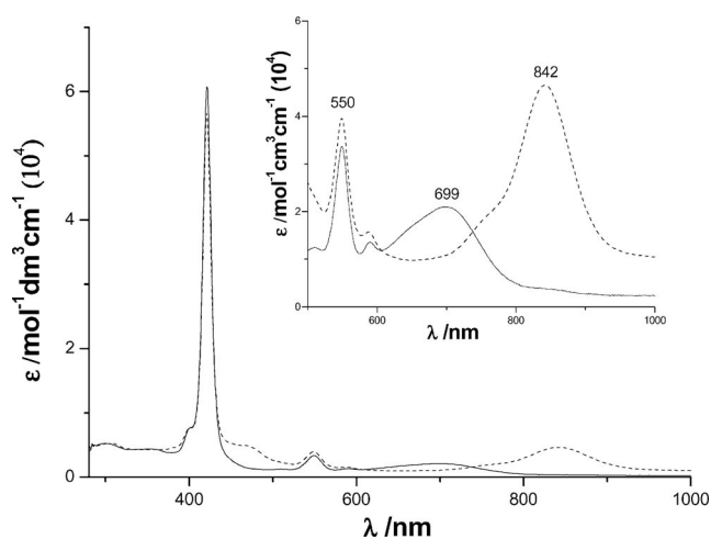
Figure 3. Absorption spectra of dyad 25 (—) and 25·H + (----) recorded in dichloromethane (concentration of 25 used was 1.97 \times 10^{-6} M). The inset shows expansion of 500–1000 nm region.
