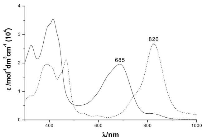
Figure 1. Absorption spectra of 21,23-dithiaphlorin 6 (—) and 6·H + (-----) recorded in dichloromethane. The concentration of 6 used was 2.34 \times 10^{-5} M.
