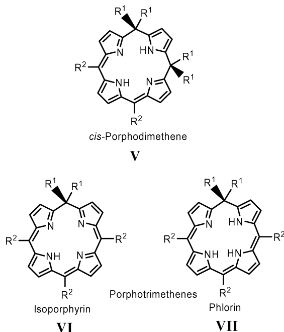
Scheme 2. Structures of calix(4)pyrins.
