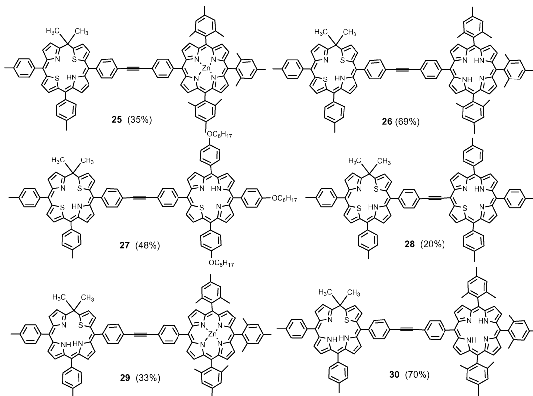
Scheme 9. Covalently linked thiaphlorin–porphyrin dyads 25–30 .
