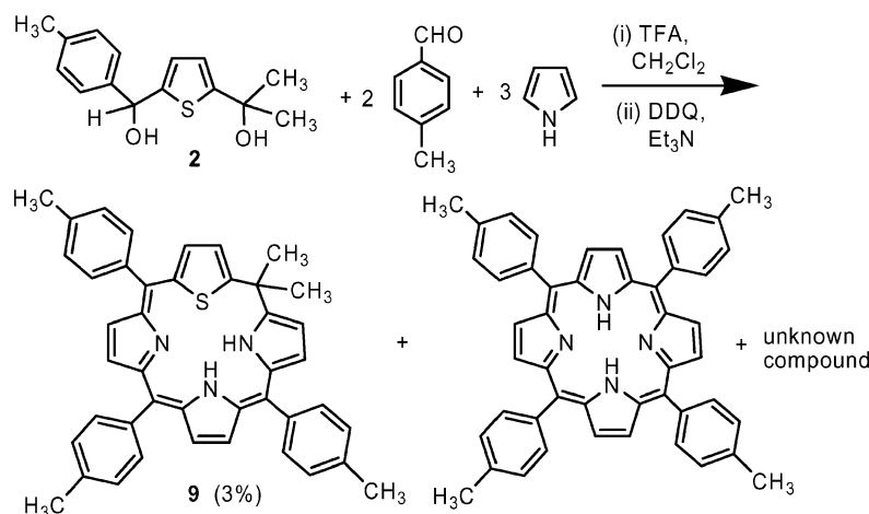
Scheme 6. Synthesis of 21-thiaphlorin 9 .
