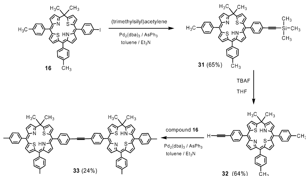
Scheme 11. Synthesis of bis(21,23-dithiaphlorin) dyad 33 .
