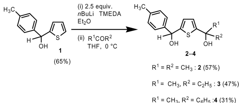
Scheme 4. Synthesis of unsymmetrically substituted 2,5-thiophenedimethanols 2–4 .
